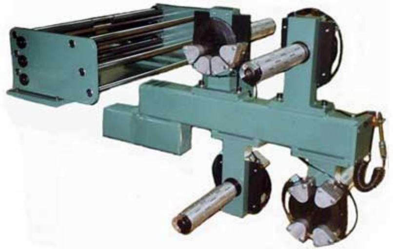
FOUR (4) PAPER ASSEMBLY TO WIND TWO (2) COILS SIMULTANEOUSLY WITH TWO (2) PAPERS PER COIL.
